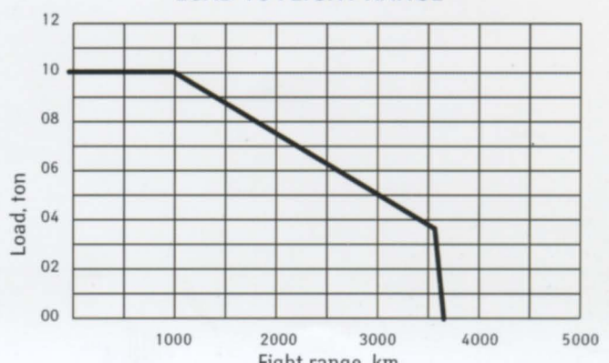
LOAD VS FLIGHT RANGE
